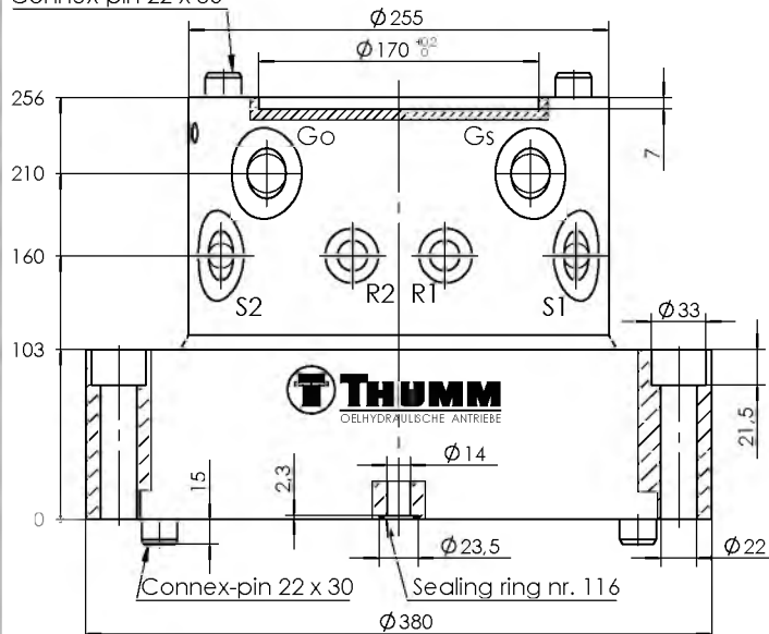
Shock valves for grab rotate
