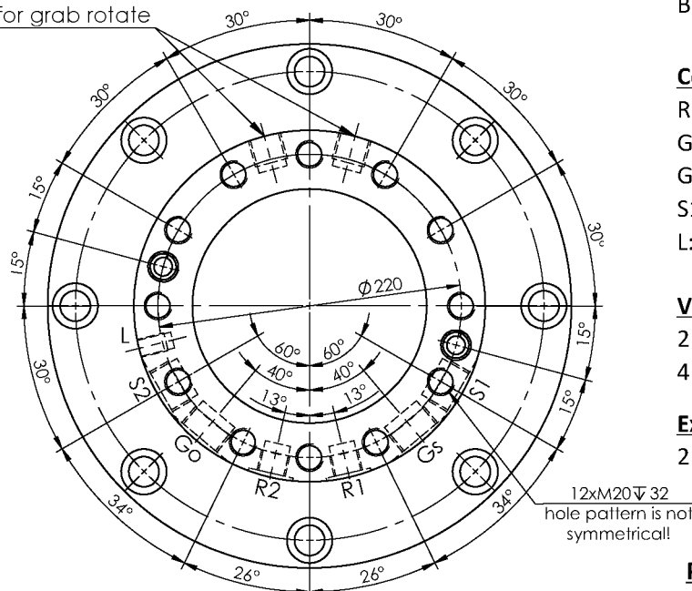
Shock valves for grab rotate
